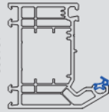
101309 67mm Outerframe
