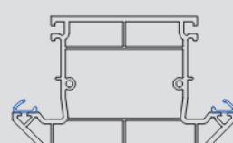
702505 116mm Midrail
