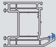
105176 80mm Outerframe
